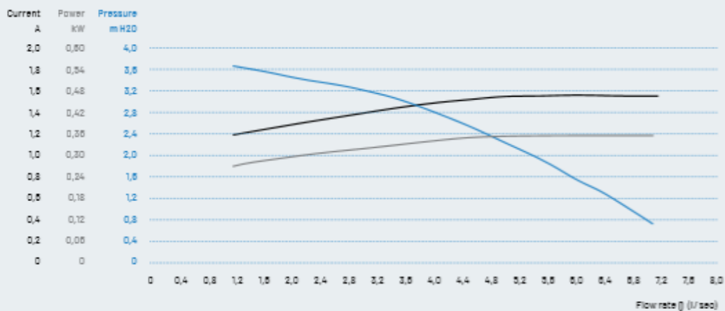
Euro Executive PF-20-2N22X low speed – Performance curves
