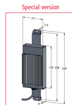
wiring cable and screw-mounting vertical
