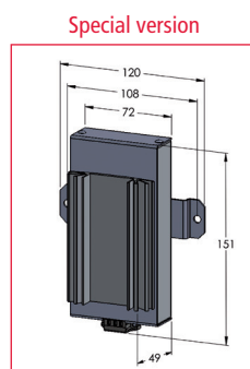
plug-in terminal and screw-mounting
