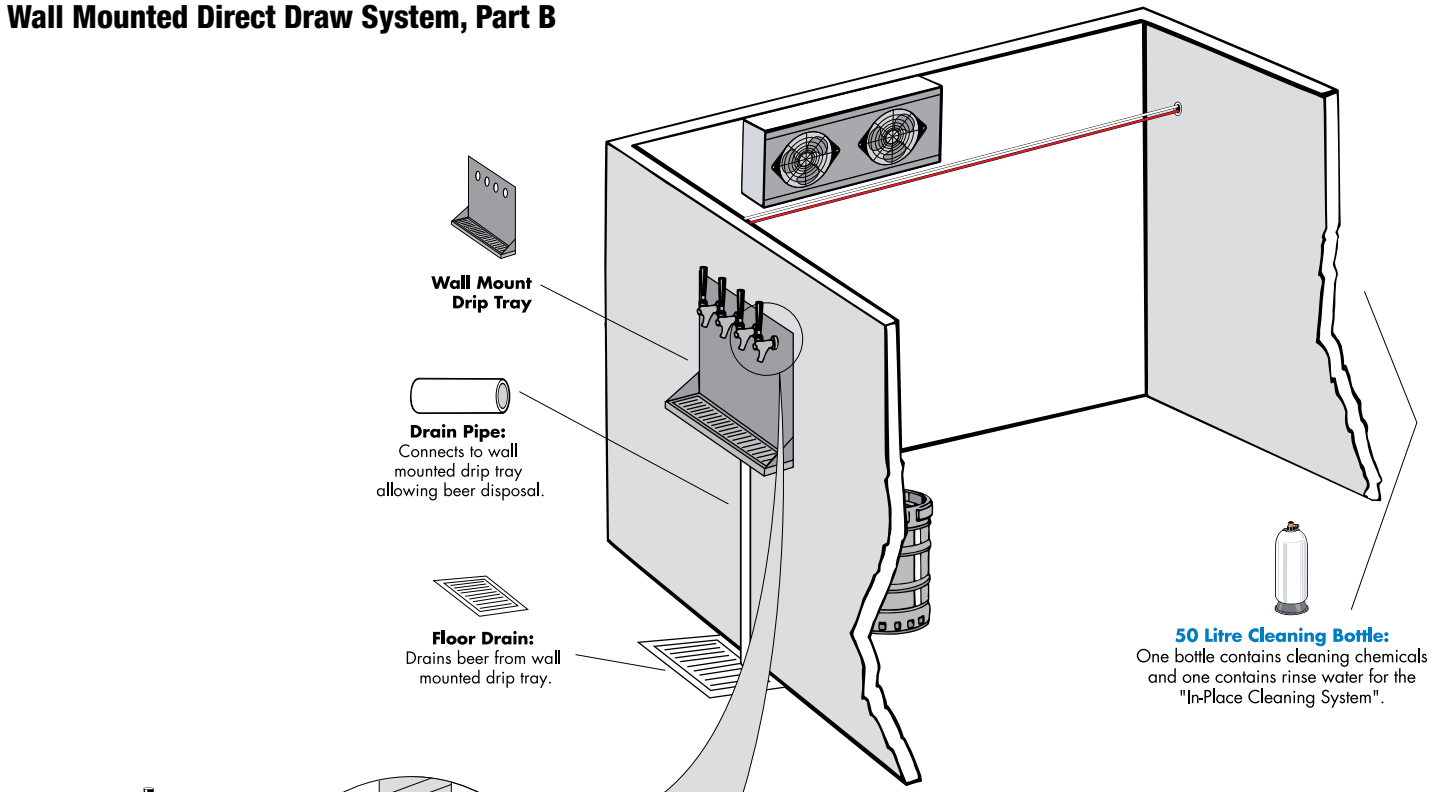
Walk-in Cooler Outside Connection View
