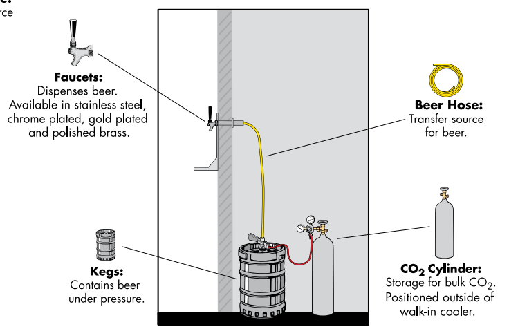
Walk-in Cooler Side Connection View
